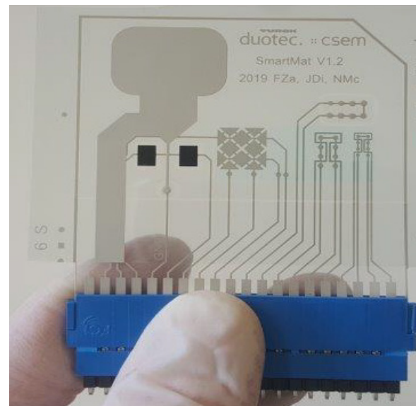
Figure 2: Pressure sensors (test features) for smart shelves (Turck duotec case).
